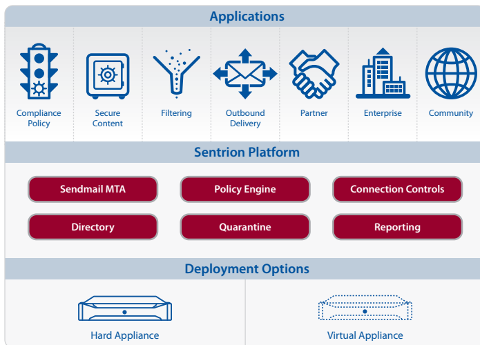
Figure 1. Sentriion Message Processing Architecture.
